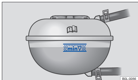
Fig. 140 In the engine compartment: markings on the coolant expansion tank (illustration).
