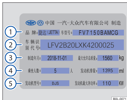
Fig. 161 Vehicle data plate (illustration)
