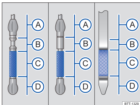
Fig. 138 Engine oil level markings on the oil dipstick (illustration)
