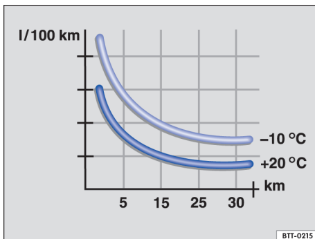
Fig. 82 Fuel consumption in litres per 100 km at two different outside temperatures.
