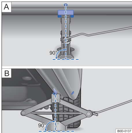
Fig. 156 Jack applied at the rear left-hand side of the vehicle
