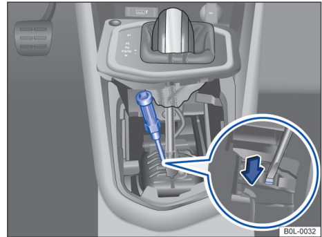
Fig. 91 Releasing the selector lever lock manually
