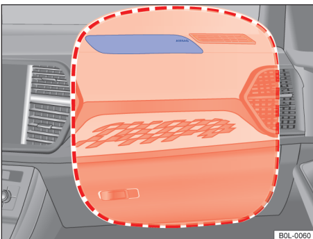
Fig. 30 Installation position and range of action of front passenger airbag
