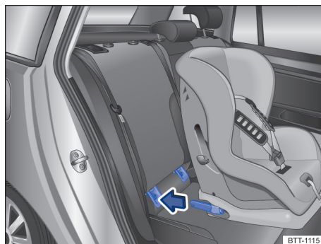
Fig. 37 Diagram: ISOFIX child seat is installed with fixed arm
